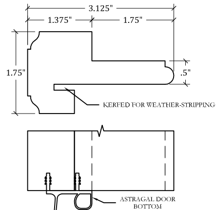
DETAIL: AST-101 ASTRAGAL
