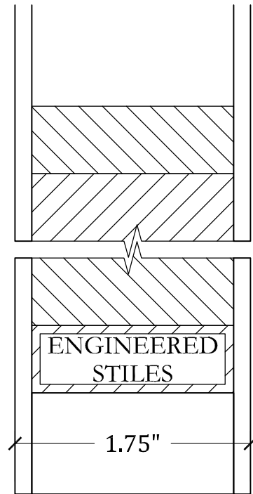
DETAIL @ EXTERIOR CORE
