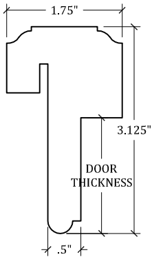
AST-301 (Interior) Drawn with 1.75" Door Thickness
