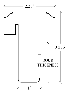
AST-401 (Exterior & Interior)
