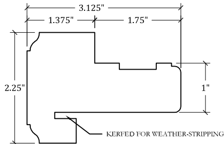
DETAIL: AST-205 ASTRAGAL FOR GU ACTIVE and INACTIVE DOORS 1" T-ASTRAGAL
