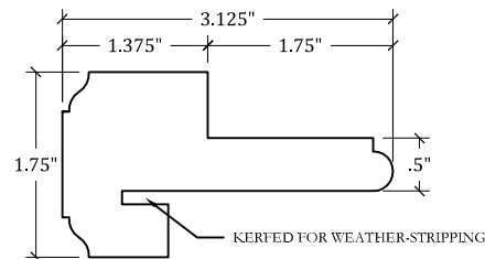
DETAIL: AST-101 ASTRAGAL
