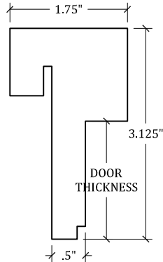
AST-305 (Interior) Drawn with 1.75" Door Thickness
