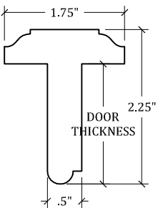
AST-301 (Interior) Drawn with 1.75" Door Thickness
