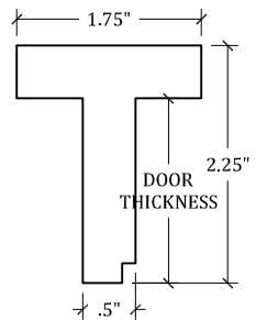
AST-305 (Interior) Drawn with 1.75" Door Thickness
