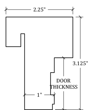
AST-206 (Exterior) Drawn with 1.75" Door Thickness
