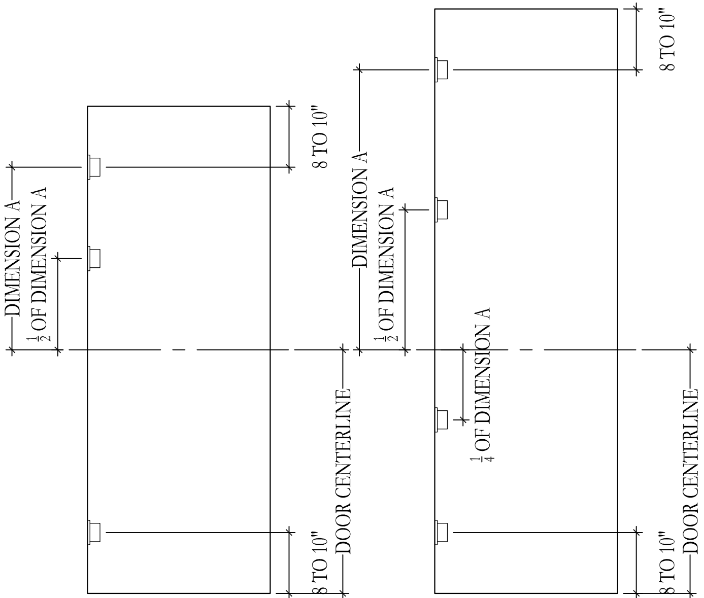
TYPICAL HINGE LAYOUTS FOR SOSS INVISIBLE HINGES
