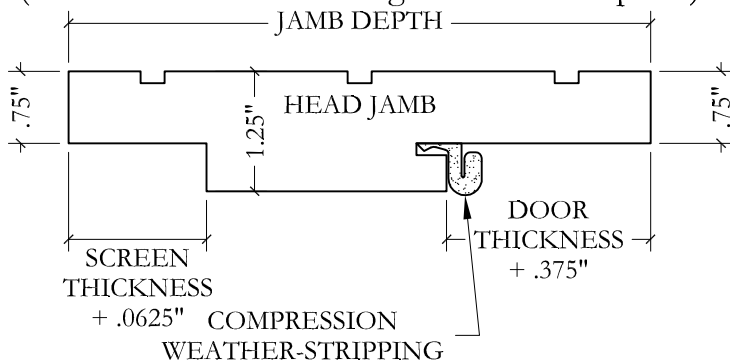
Double Rabbeted Jamb with Q-Lon (Exterior Standard Inswing with Screen Option)
