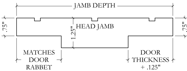
Double Rabbeted Jamb
