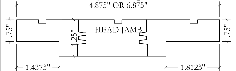
20 Minute Fire Rated Single Rabbeted Jamb (Double Rabbeted is Also Available)
