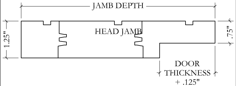
Double Rabbeted Finger Jointed Jamb Jambs Come with Specific Rabbet Depths This Restricts Jamb Depths Available.
