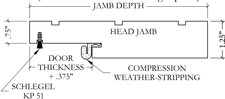
Single Rabbeted Jamb with Q-Lon and Secondary Weatherstripping (Exterior Standard Outswing Option)
