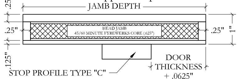
45 or 60 Minute Fire Rated Flat Jamb with Applied Stop
