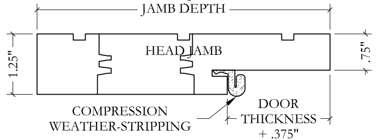
Single Rabbeted Duraframe Jamb with Q-Lon
