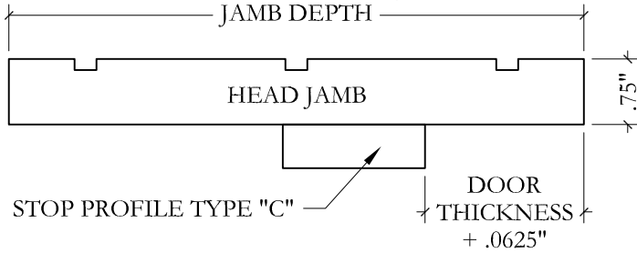
Flat Jamb with Applied Stop (Interior Standard Option)
