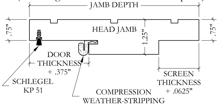
Double Rabbeted Jamb with Q-Lon and Secondary Weatherstripping (Outswing Door With Screen/Storm Option)
