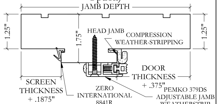
Double Rabbeted Jamb with Q-Lon and Screen/Storm Weatherstripping (Impact/Coastal Standard Inswing with Screen Option)
