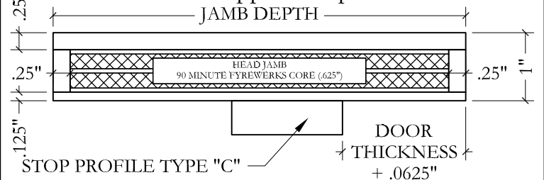
90 Minute Fire Rated Flat Jamb with Applied Stop
