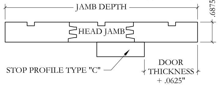
Flat Finger Jointer Jamb with Applied Stop
