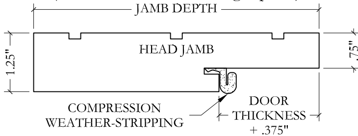
Single Rabbeted Jamb with Q-Lon (Exterior Standard Inswing Option)
