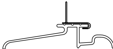
PEMKO 145 INTERLOCK w/ PAN & J-HOOK FOR INSWING ONLY
