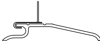
PEMKO 110 INTERLOCK w/ PAN & J-HOOK FOR OUTSWING ONLY
