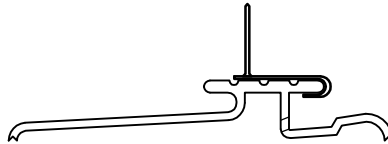
PEMKO 142 INTERLOCK w/ PAN & J-HOOK FOR INSWING ONLY
